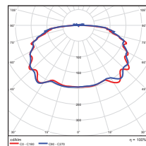
42 Watt Slim Lens
