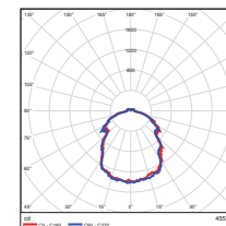
42 Watt Tall Lens
