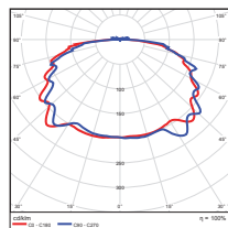
28 Watt Slim Lens
