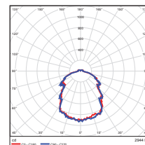
28 Watt Tall Lens
